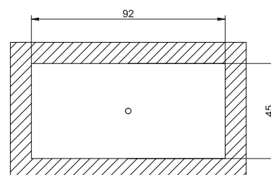
Panel Cutout
